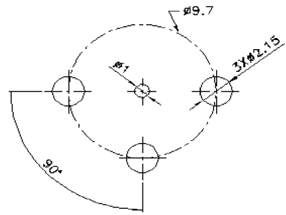
MOUNTING HOLES (印刷电路板架設孔)
