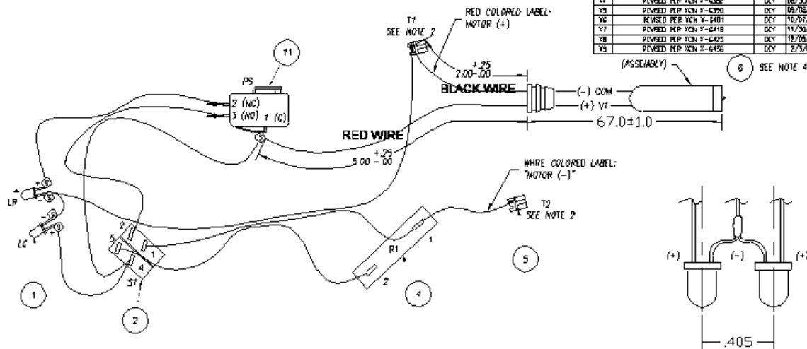
HARNESS LAYOUT SCALE: NTS
