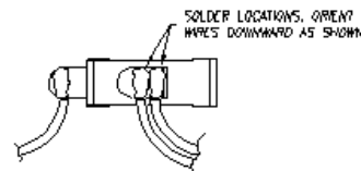
SWITCH DETAIL SCALE: NTS
