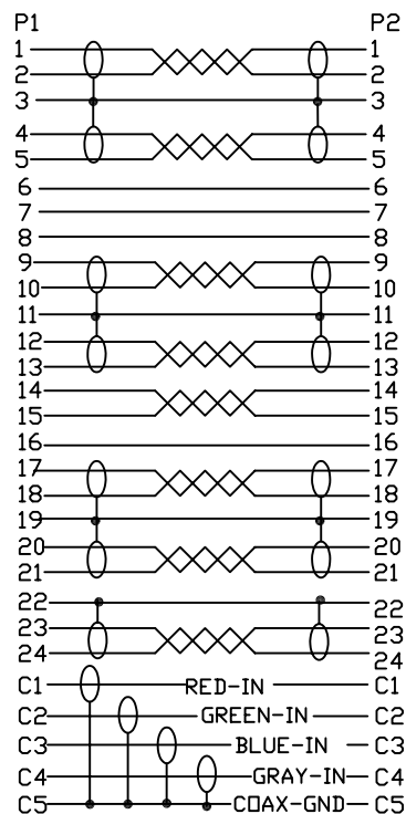
PIN ASSIGNMENT
