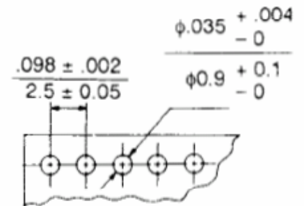
P.C. Board Hole Dimensions
