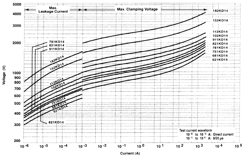
V-I Curve (621K to 182K)
