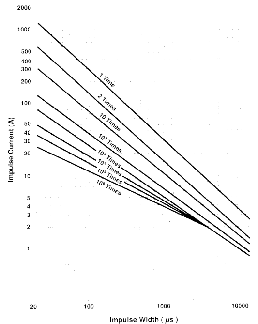
V-I Surge Life Time Ratings (820K to 821K)
