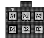
Rear View Crimp/wire insertion side
